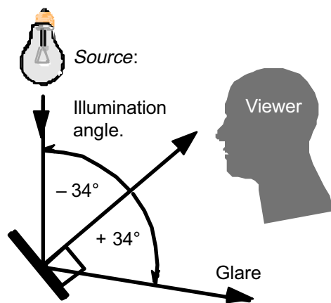
Figure 3. Optimum design angle for incidence of source illumination on the display is 34^\circ as determined by tests based on variations in overhead lighting and comfortable head positions. It is assumed that the preferred viewing angle is perpendicular to the display. Illumination angles are measured from the normal. Source-normal angle is defined to be negative.
