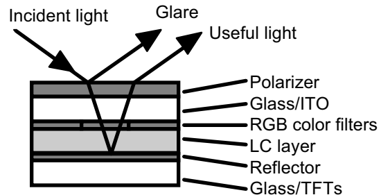
Figure 1. Simplified stackup of a reflective color LCD with an internal reflector [2]. Total reflected light is about 8% of the incident light. Note that the reflected light, useful for viewing the display, is aligned with glare making the display unreadable where the reflected useful light is maximum. [The diffuser is not shown for clarity]
